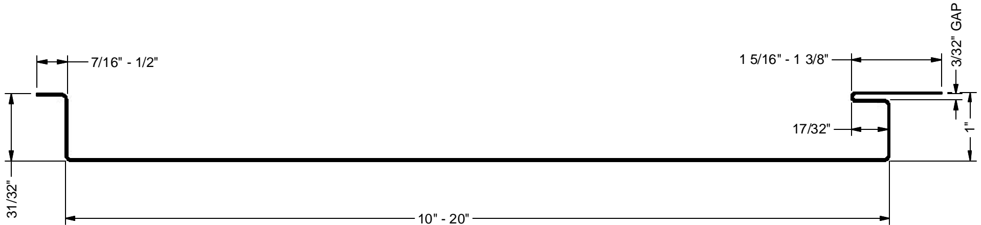
PANEL SHOWN WITHOUT PERFORATIONS
